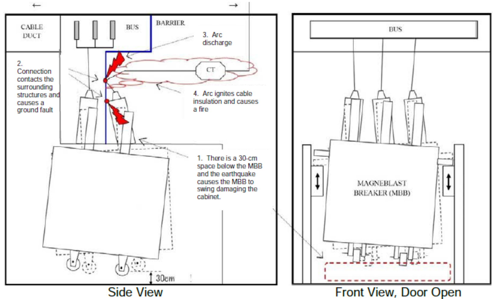
Figure 1.2-2. Onagawa Arching Scenario
